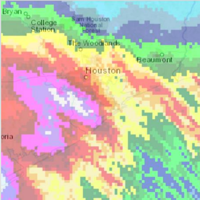
8/29 Radar
