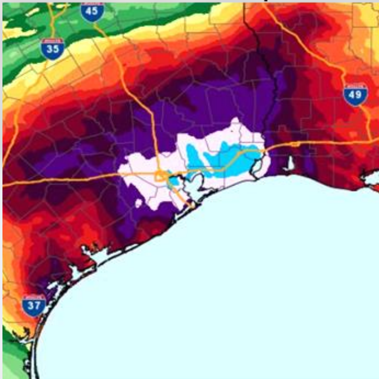
9/1 Observed Rainfall
