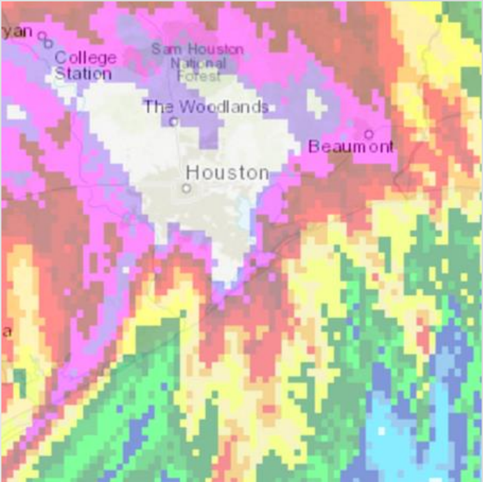
8/30 Radar
