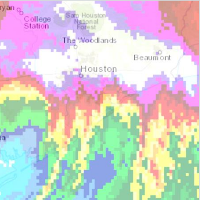
8/31 Radar
