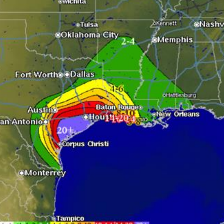
8/26 Rainfall Forecast
